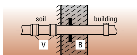
SML pipe with wall flange
