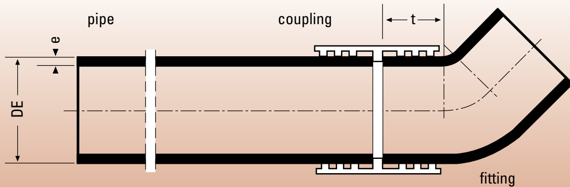
Construction dimensions:
