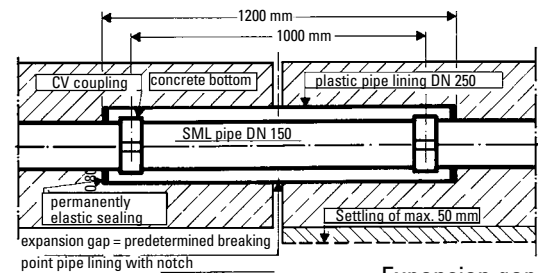
Expansion gap
